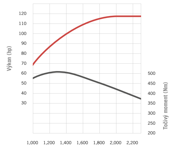
Farmall 120 C
