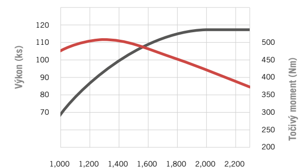
Farmall 120 C
